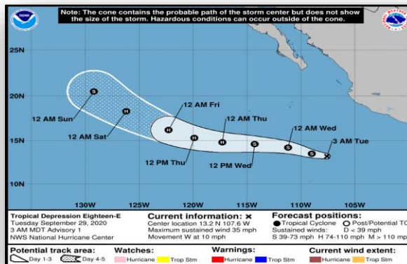
Eastern Pacific
