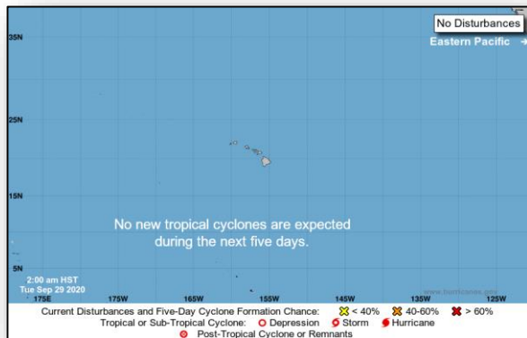
Central Pacific
