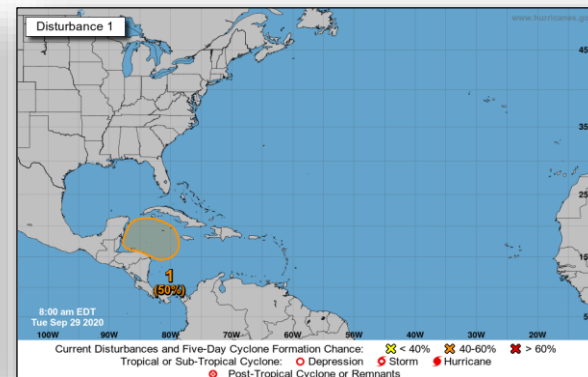
Atlantic
