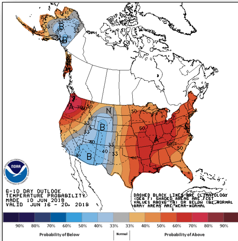
Temperature Probability
