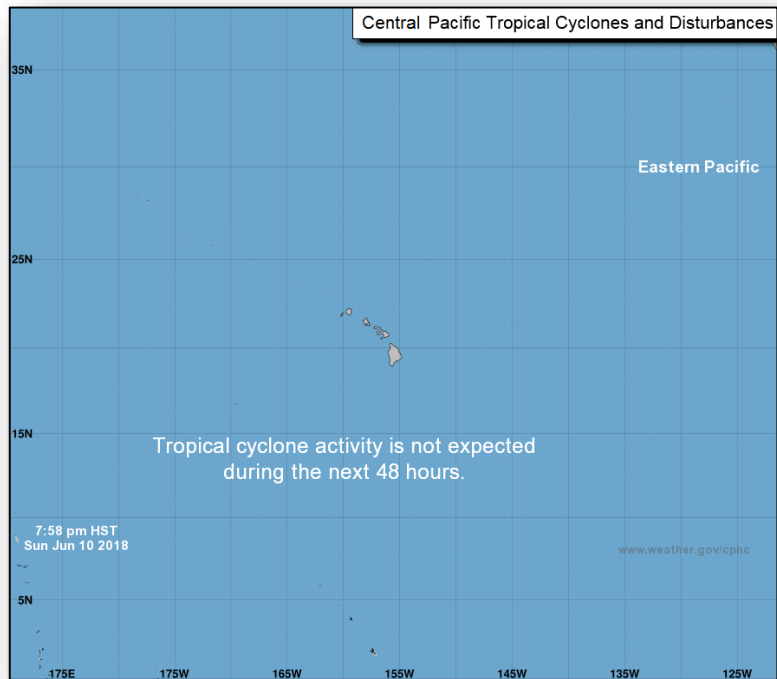
48 Hour Outlook
