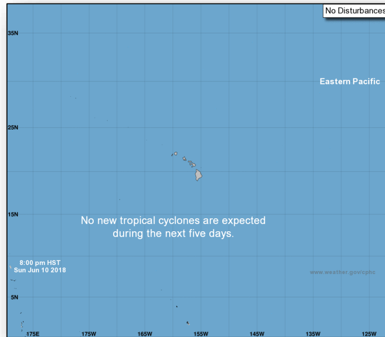
5 Day Outlook
