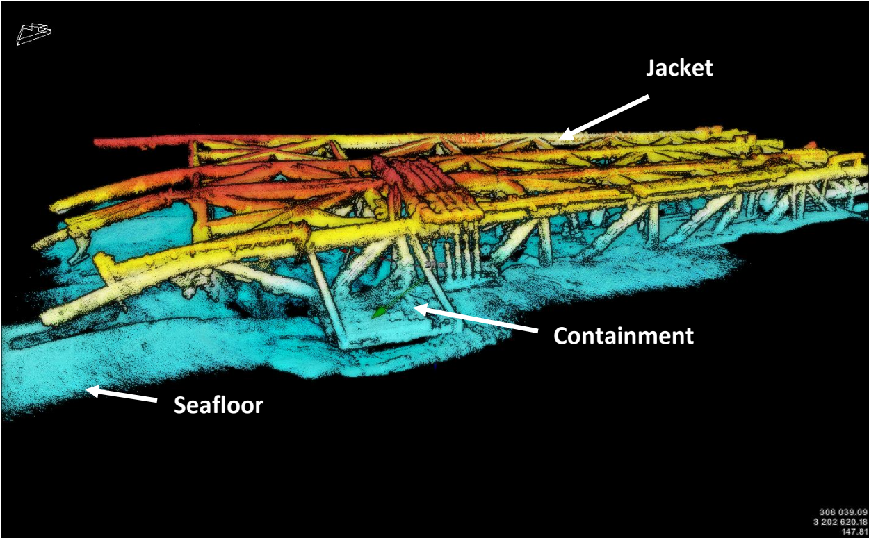
Echoscope image of containment system fully installed – no plumes coming from the erosional pit
