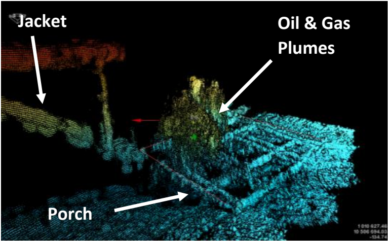
Echoscope image of porch installed with plumes coming through without the containment device installed
