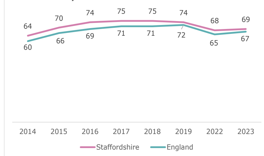
GLD Trend Analysis
