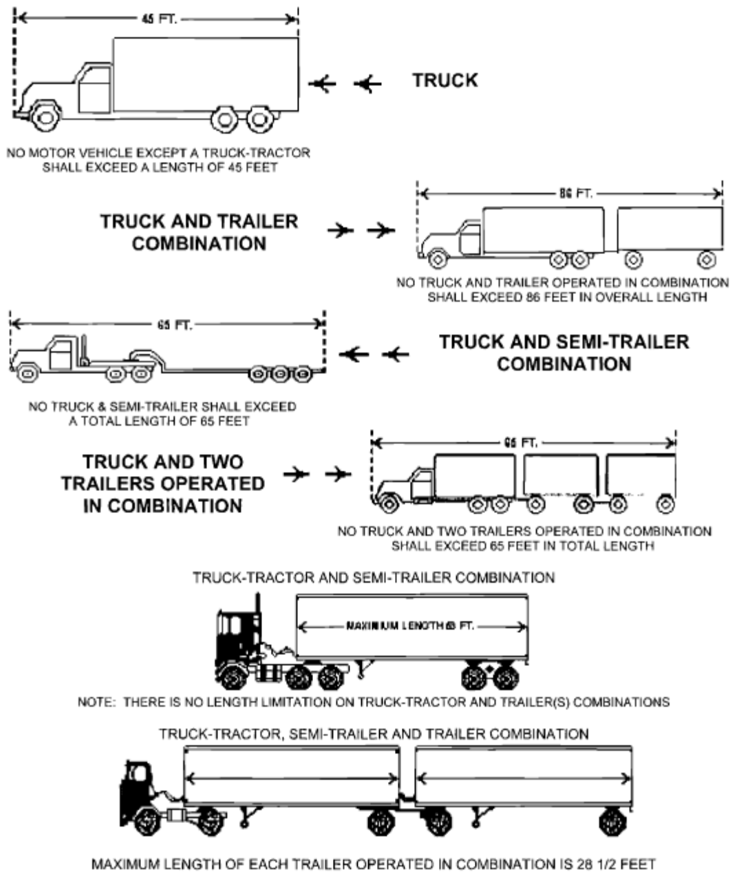
Figure 2-2 Maximum Sizes
