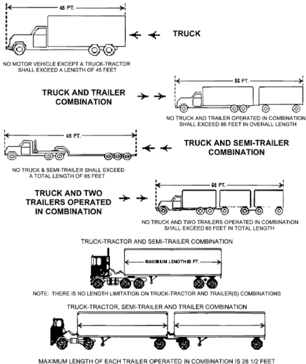
Figure 2-2 Maximum Sizes
