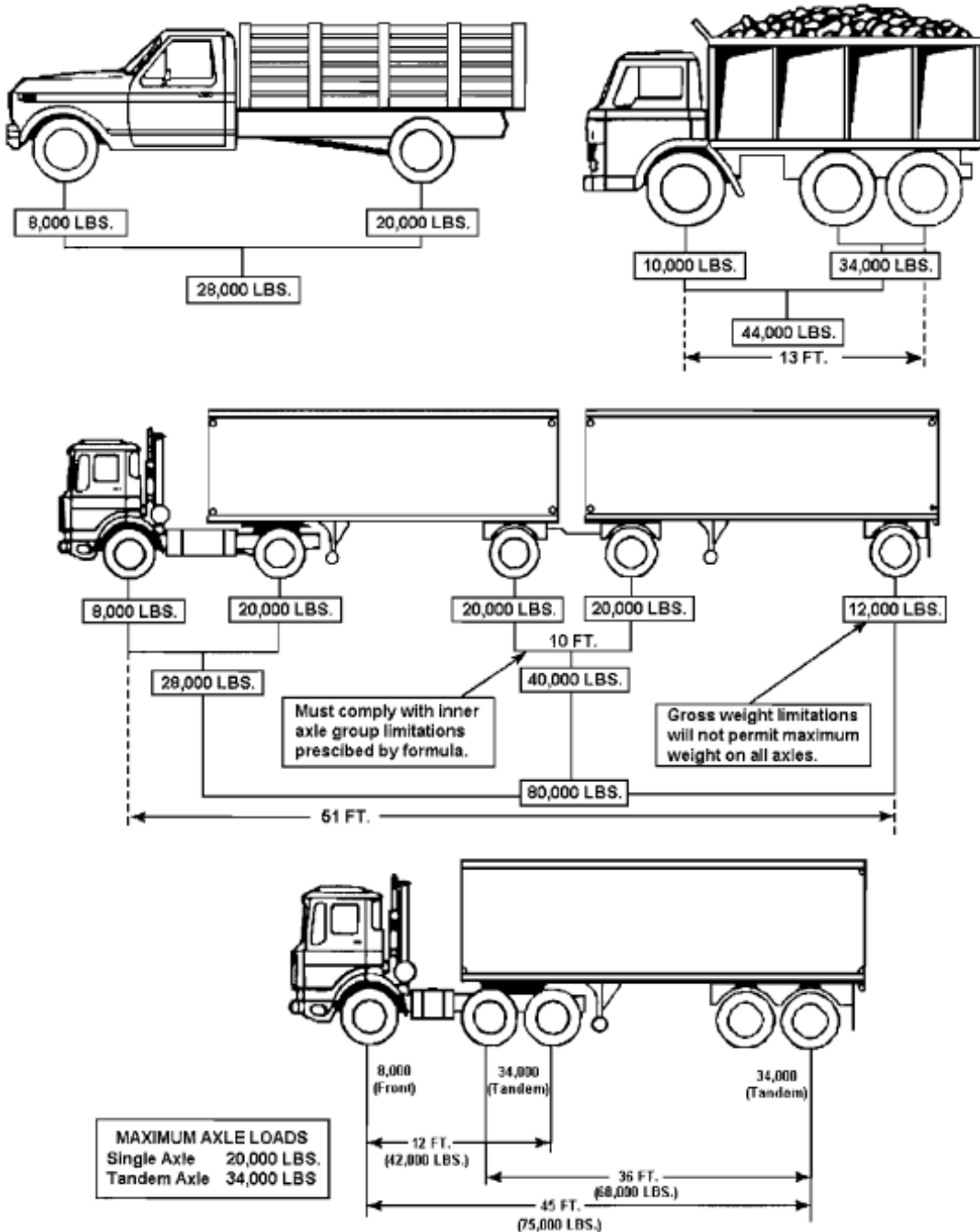
Figure 2-1 Maximum Weights
