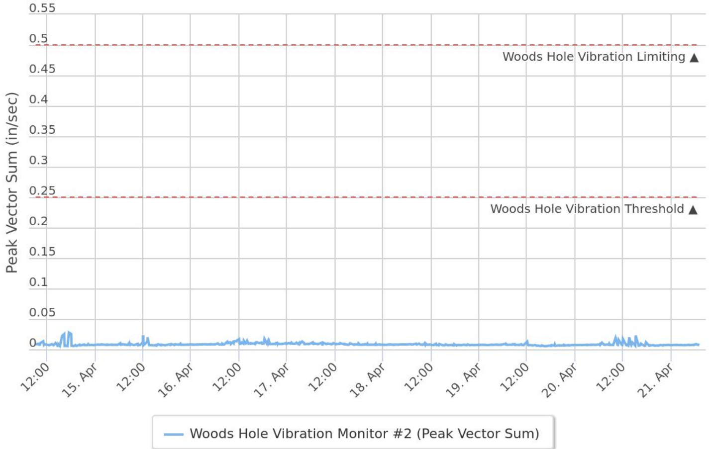
Peak Vector Sum (in/sec) April 14, 2021 - April 21, 2021
