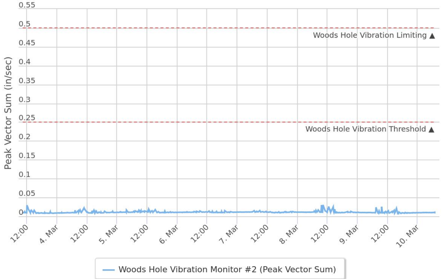
Peak Vector Sum (in/sec) March 3, 2021 - March 10, 2021
