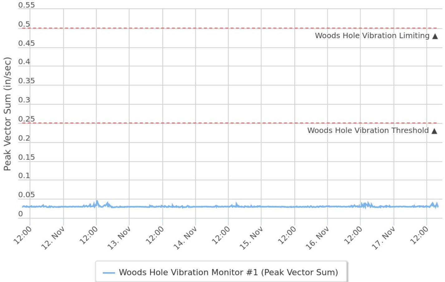
Peak Vector Sum (in/sec) November 11, 2020 - November 18, 2020
