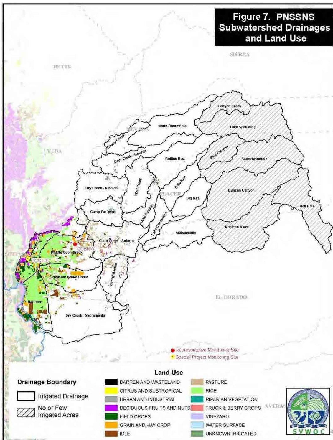
Figure 67 - PNSSNS Subwatershed Drainages and Land Use
