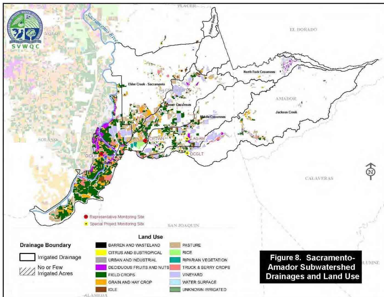
Figure 78 - Sacramento-Amador Subwatershed Drainages and Land Use
