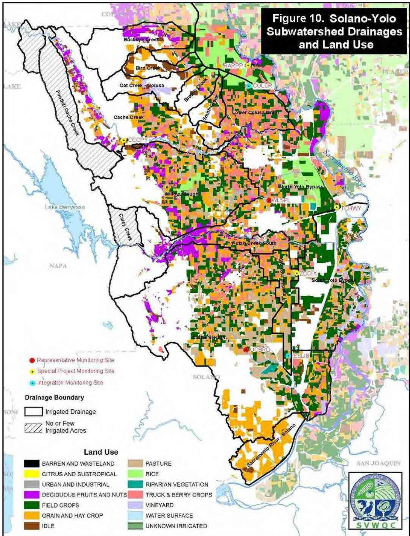
Figure 910 - Solano-Yolo Subwatershed Drainages and Land Use
